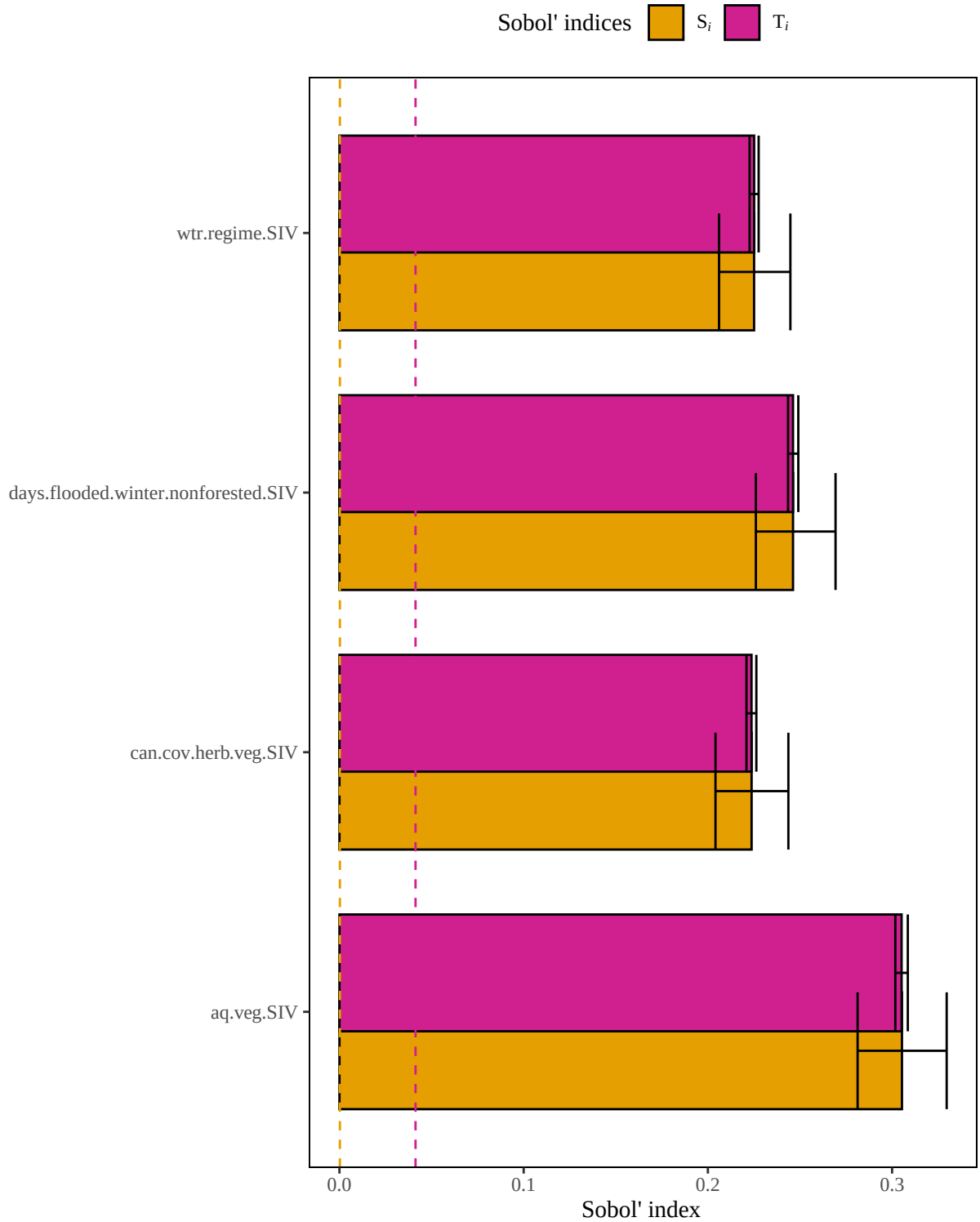
Figure 4. Results of a sensitivity analysis for the mallardNonforestedPaluLacRiv model based on an arithmetic mean structure. Dashed lines represent baseline numerical approximation error for S_i and T_i ( i.e. , dummy variables).
